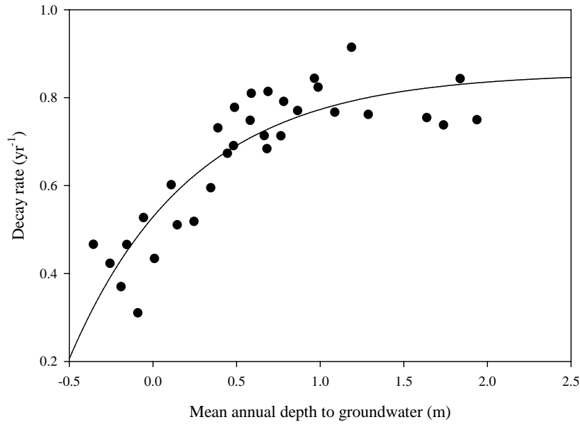
Fig. 11 Asymptotic regression for mean decay rates (yr -1 ) vs mean annual depth to groundwater ( r^2=0.78 p<0.001 ). Groundwater values are from the Dupuit method.
